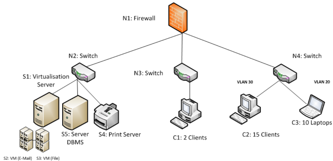
Figure 2: Excerpt of a network plan (RECPLAST Subnetwork A)
